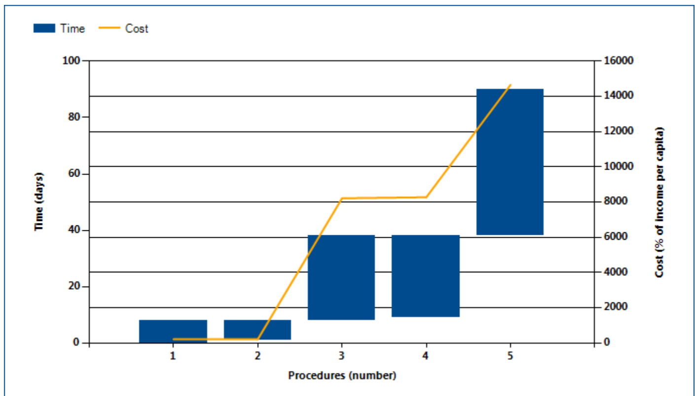
Figure 4.1 What it takes to obtain an electricity connection in Benin -
