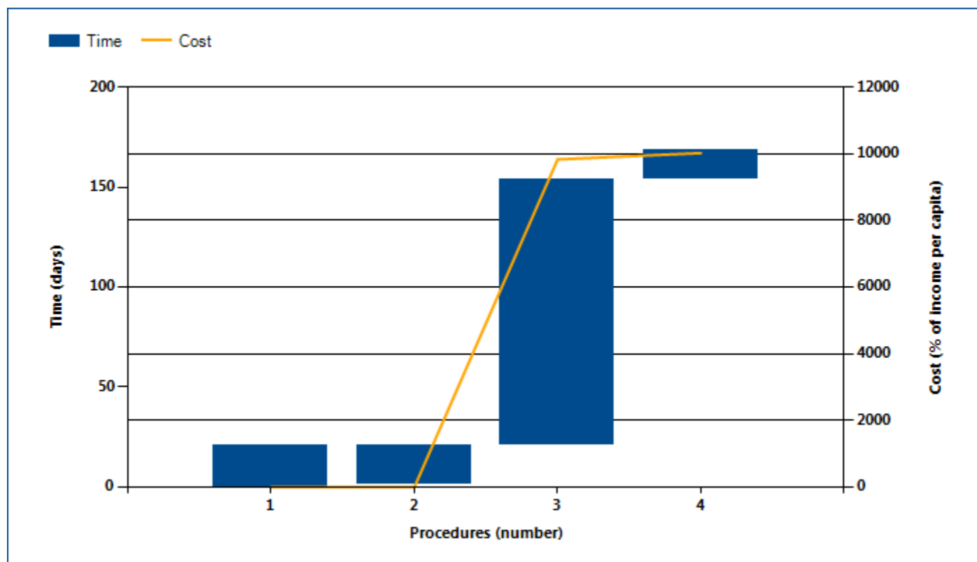
Figure 4.1 What it takes to obtain an electricity connection in Burkina Faso
