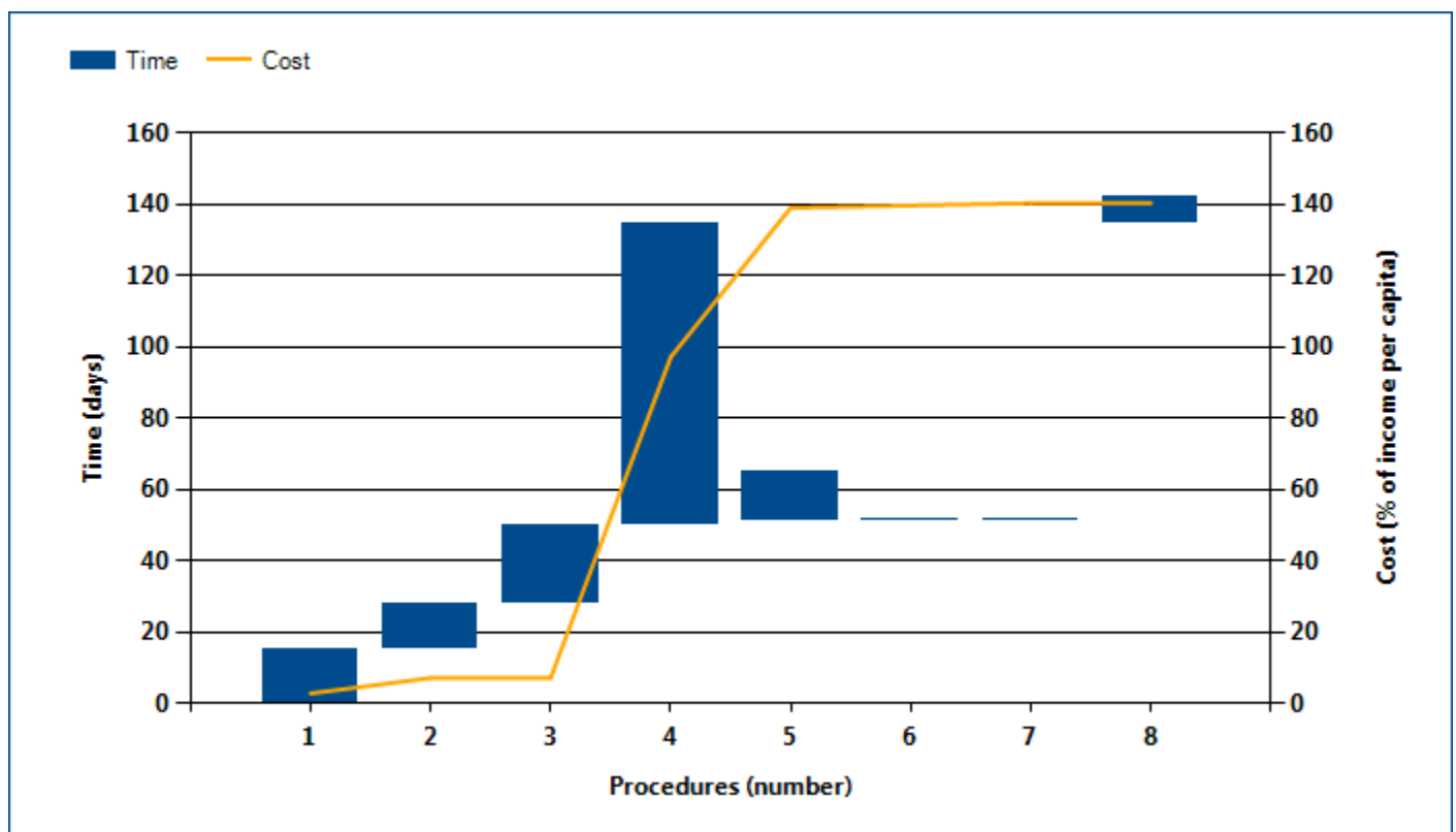
Figure 4.1 What it takes to obtain an electricity connection in Canada
