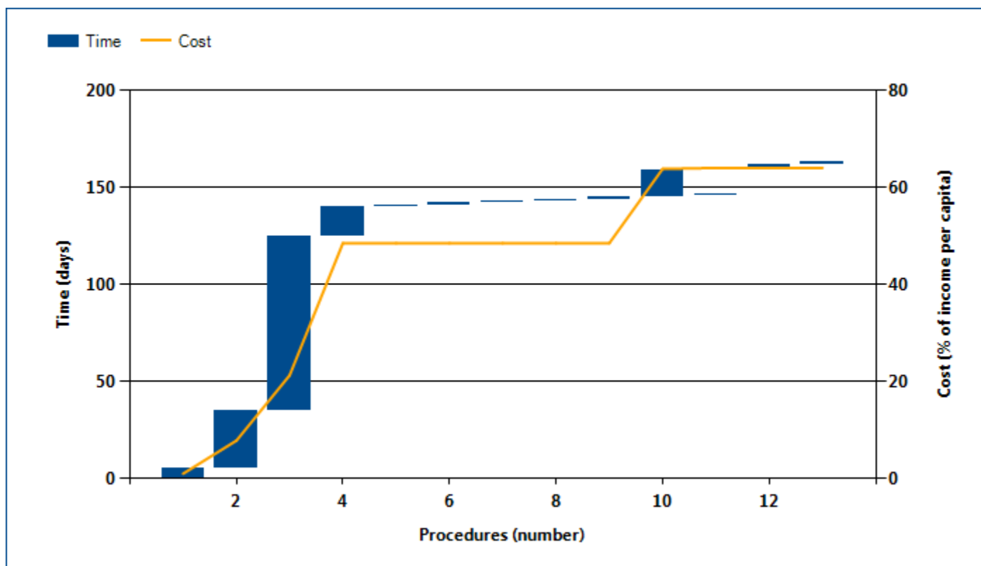
Figure 3.1 What it takes to comply with formalities to build a warehouse in Canada
