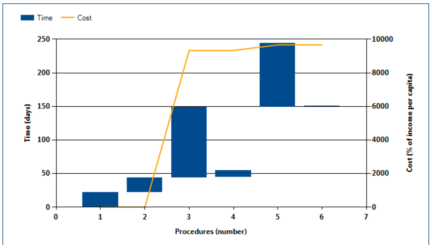
Figure 4.1 What it takes to obtain an electricity connection in Malawi
